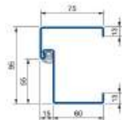
Blockzarge 95/75
