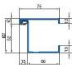
Blockzarge 62/75
