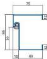
Blockzarge 85/75 Standard
